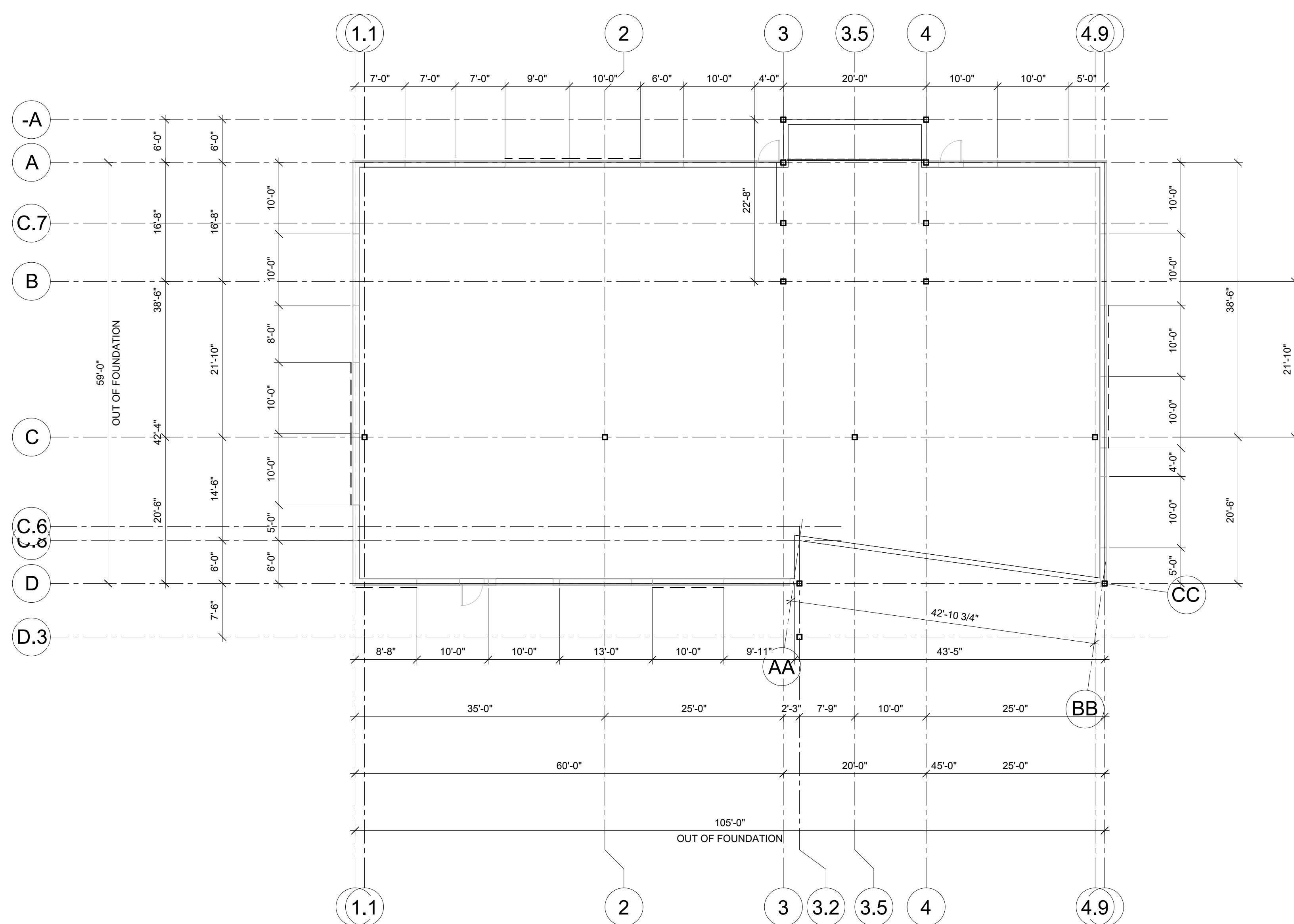
ANCHOR PLAN 3/32" = 1'-0"
