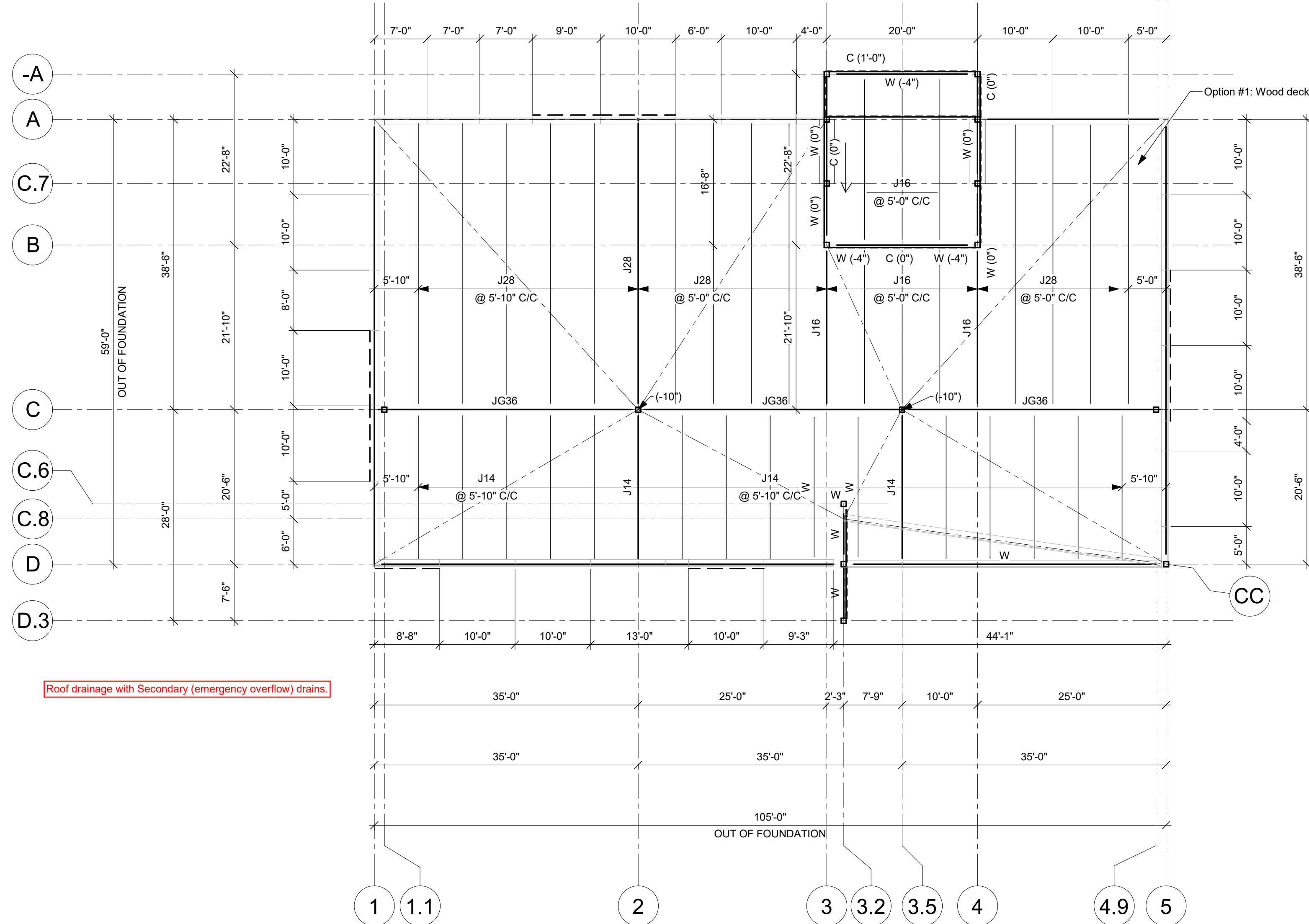
ROOF PLAN 3/32" = 1'-0"
